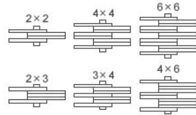
Plate Lacing
